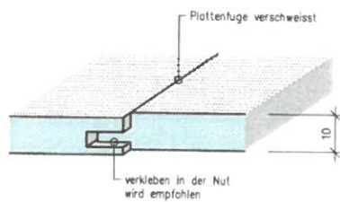
Detail "Nut/Feder"
