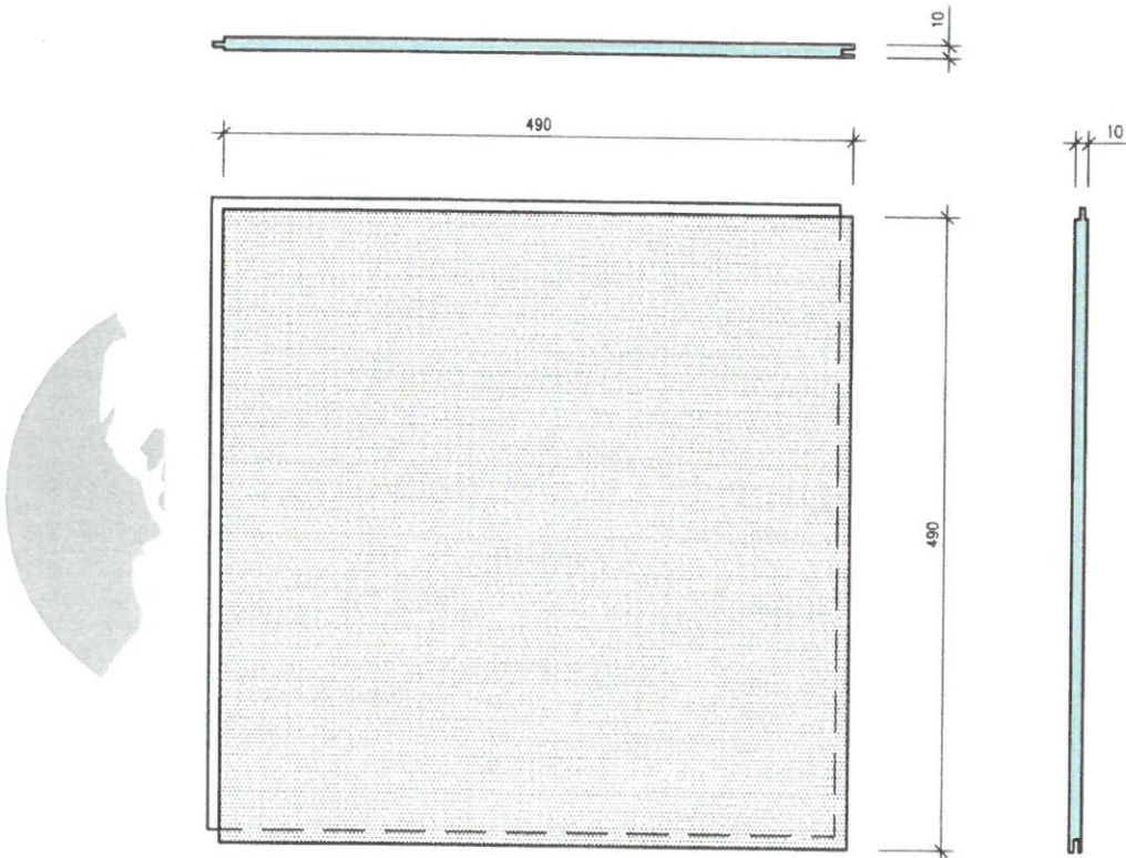
Detail "Nut/Feder"
