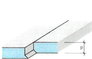
Detail "plus"- Verriegelung
