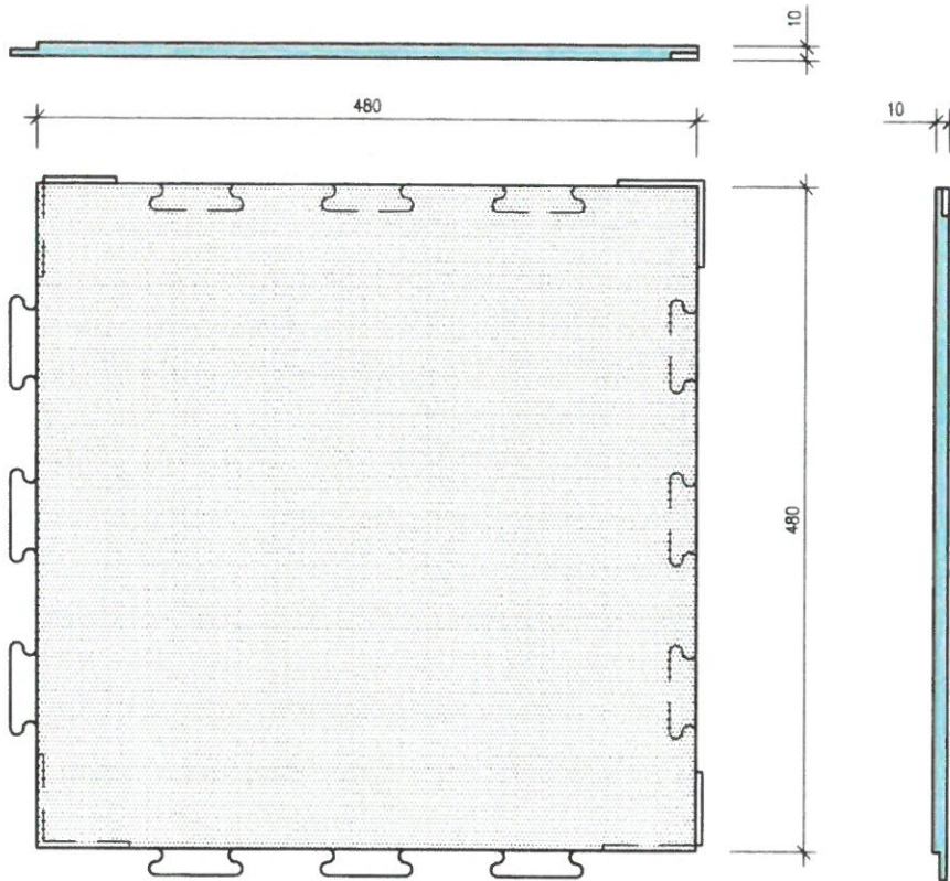
Detail "plus"- Verriegelung
