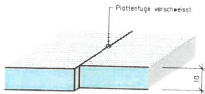
Fugendetail
